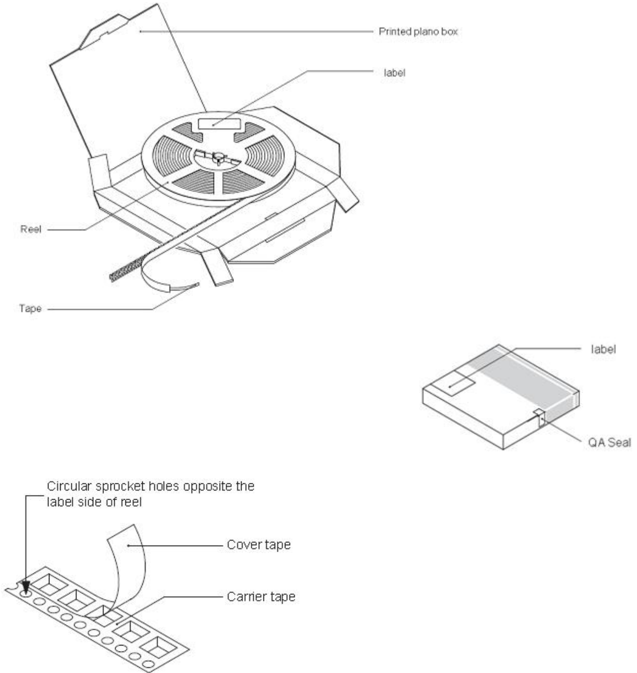
Fig.1- Reel pack for SOD882
