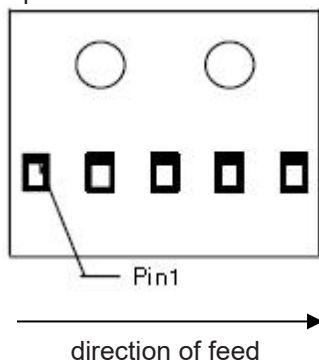
Fig 2. Product orientation in carrier tape
